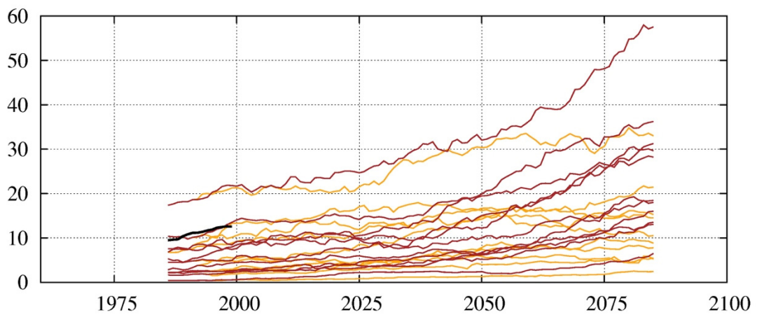
Fig. A11 Projected mean number of hot days (time series of individual simulations) during the growing season (in days) for regions E (top), NW (middle), and SW (bottom). Shown are all individual model simulations contributing to the ensemble (RCP4.5 in yellow, RCP 8.5 in red) smoothed by a 30-year running mean referenced to the period 1971-2000. Time axis values represent the mid-year of a 30-year period. The black line shows observational E-OBS data, likewise averaged over a 30-year period.
