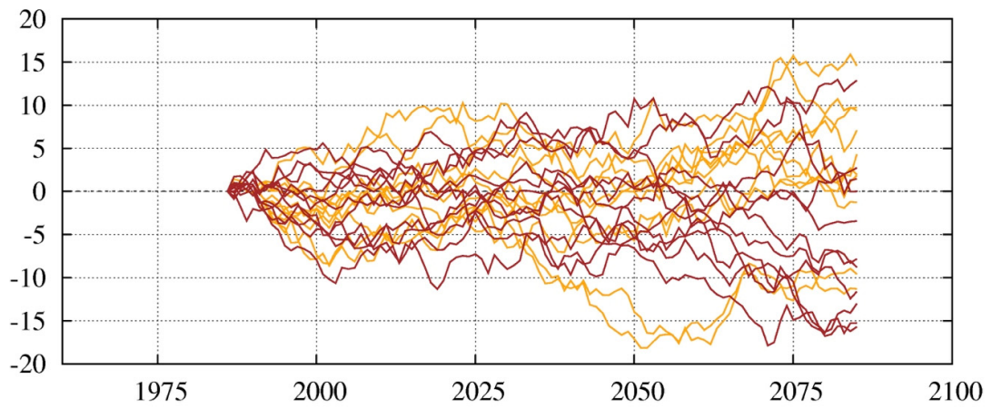
Fig. A2 Projected changes in mean precipitation sum (time series of individual simulations) during the growing season (in %) for regions E (top), NW (middle), and SW (bottom). Shown are all individual model simulations contributing to the ensemble (RCP4.5 in yellow, RCP 8.5 in red) smoothed by a 30-year running mean referenced to the period 1971-2000. Time axis values represent the mid-year of a 30-year period.
