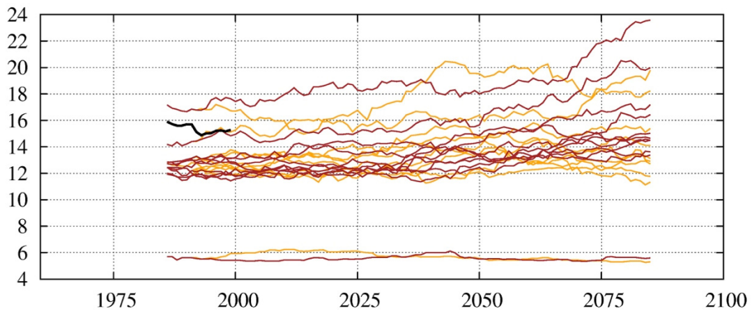
Fig. A9 Projected mean maximum duration of dry spells (time series of individual simulations) during the growing season (in days) for regions E (top), NW (middle), and SW (bottom). Shown are all individual model simulations contributing to the ensemble (RCP4.5 in yellow, RCP 8.5 in red) smoothed by a 30-year running mean referenced to the period 1971-2000. Time axis values represent the mid-year of a 30-year period. The black line shows observational E-OBS data, likewise averaged over a 30-year period.
