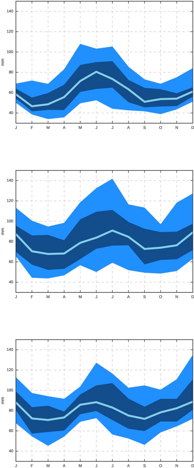
Fig. C1 Projected mean monthly precipitation sums in the 2050s (ensemble) (in mm) for regions E (top), NW (middle) and SW (bottom). Displayed are the ensemble median (light blue line), the likely range (dark blue shaded area), and the ensemble range (light blue shaded area).
